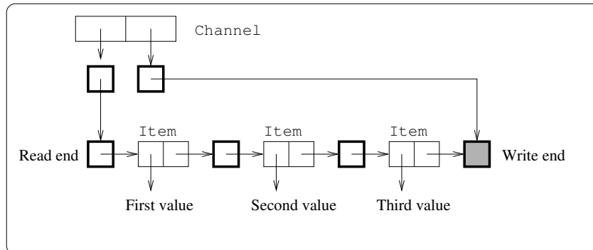
Fig. 10. Structure of the buffered channel implementation
