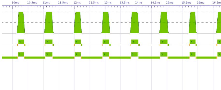
Fig. 3. Sudoku3 (zoomed) ThreadScope profile
