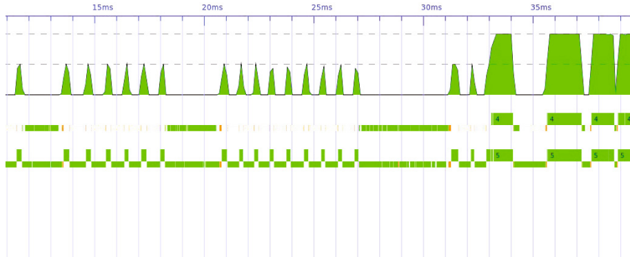
Fig. 4. Sudoku4 ThreadScope profile
